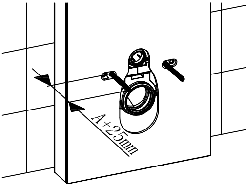
把螺杆安装到机架上 screw the bolts into the cistern frame
