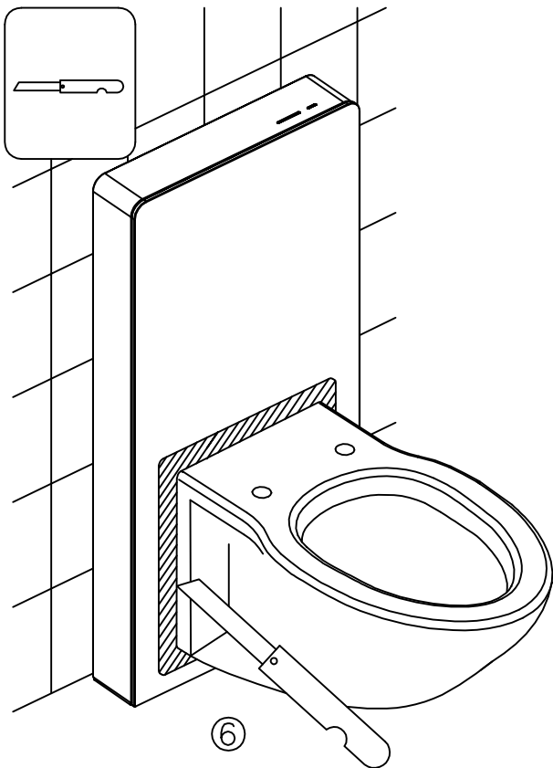
⑥ 割除多余的马桶缓冲垫 cut off extra part of the toilet mat
