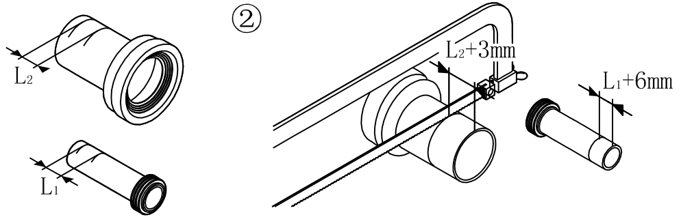
裁剪冲水直管和排水直管 cut the flush pipe and drainage pipe
