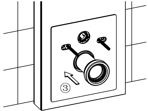
把排水直管安装到机架上 install the flush pipe onto the cistern
